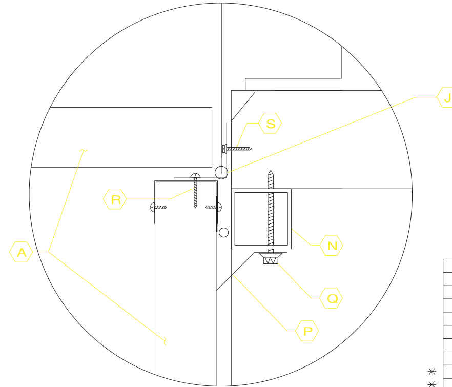
DETAIL C-C
